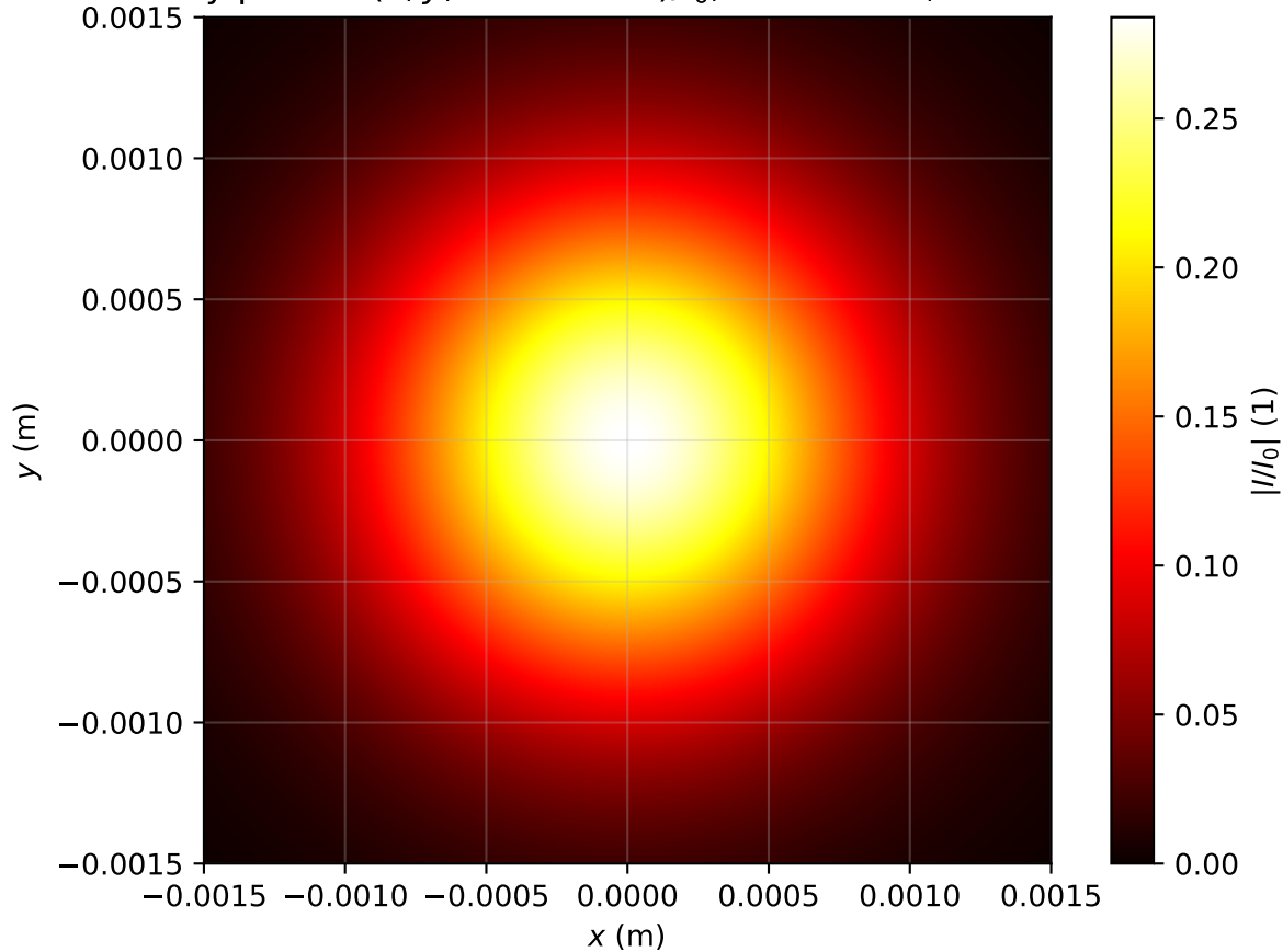
Intensity profile I(x, y, z = 3.981m)/I_0 , P_{in}=0.3P_{cr} , artificial time
